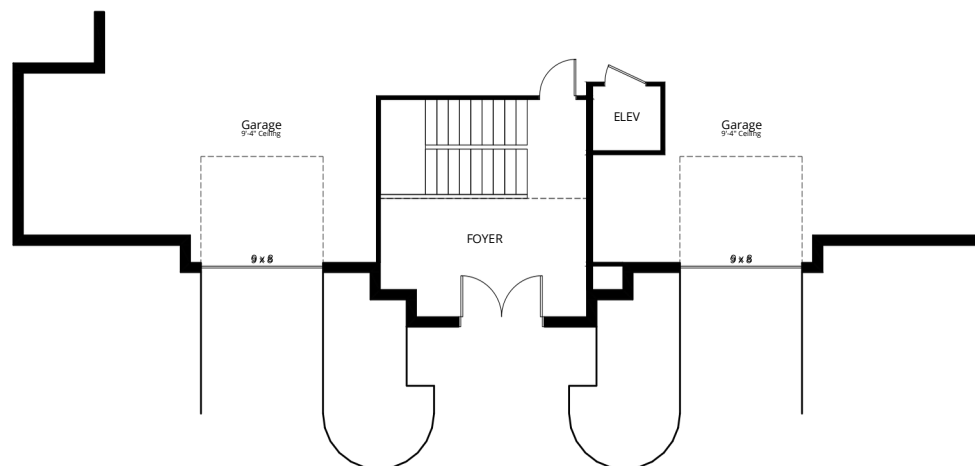
ENTRY LEVEL FLOORPLAN
